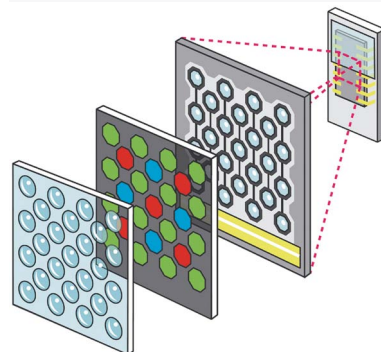
Figure 2 A diagram of a CCD sensor.
