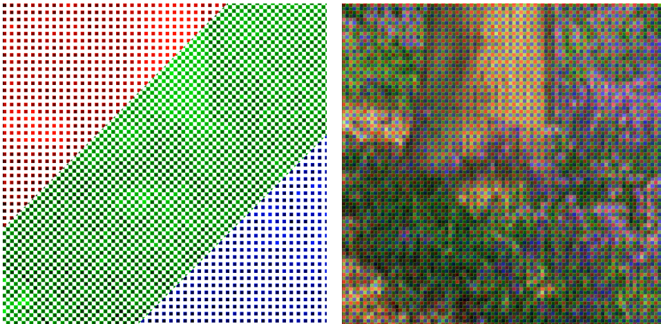
Figure 7 Let's now analyze more closely the way a one shot camera captures and interprets color using the Bayer pattern arrangement with most CCD and CMOS sensors. The sensor is simultaneously able to capture red, green and blue color. But there is only one red sensor element for every four pixel sensors. Likewise, there is only one blue sensor and there are two green sensors. The right hand picture gives some indication in close-up of how a CCD/CMOS chip captures the RGB data using this pattern of colored pixel sensors. The capture data must next be interpreted in order to produce a smoother looking result. Since only one in four pixel sensors is recording red or blue information, the values for the other three pixels (75%) has to be guessed. Although in the case of the green information, only 50% has to be guessed. Once the raw image has been processed, the underlying pattern is not seen. However, you should be aware that in the case of most one shot cameras, two thirds of the color information is guesswork. The weakness of one-shot cameras can sometimes be seen in a capture of a subject containing lots of sharp detail. Sometimes you get to see Christmas tree type artifacts, which is a result of the pixel guesswork having to fill in the gaps.
